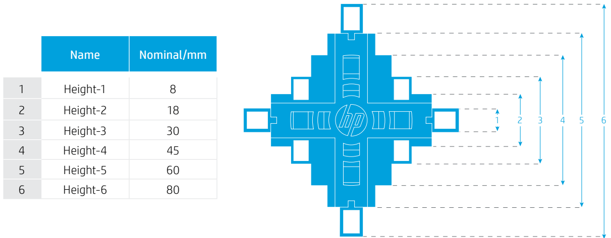
Figure 3. Diagnostic part critical dimensions
